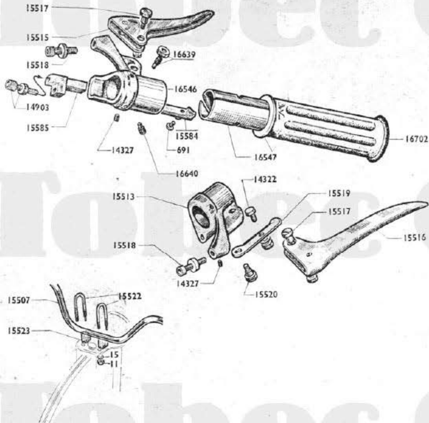
Guidon complet 15506
